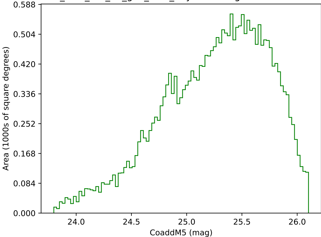
too_elab_r16_d3_griz_v3.4_10yrs Yr 3-4 g band: CoaddM5
