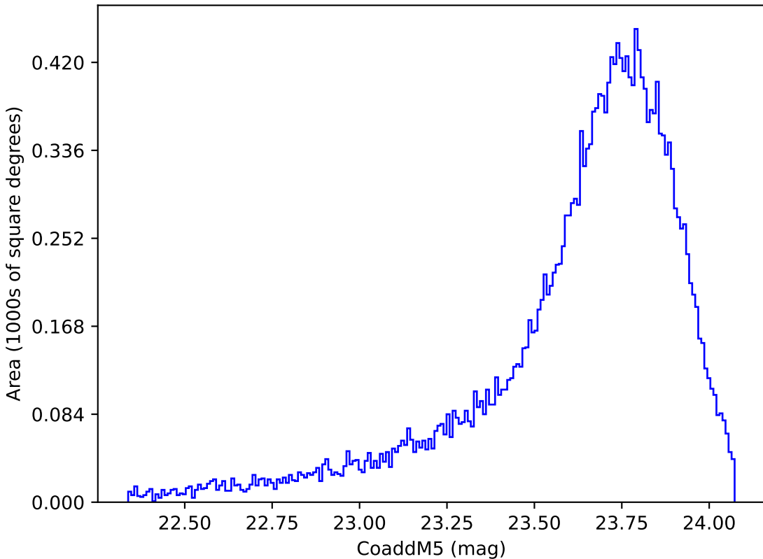
too_elab_r16_d3_griz_v3.4_10yrs Yr 1 y band: CoaddM5
