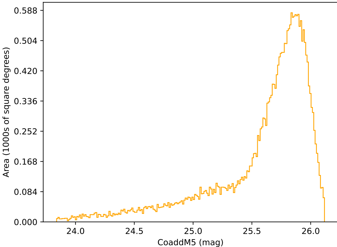
too_elab_r16_d3_griz_v3.4_10yrs Yr 1 r band: CoaddM5
