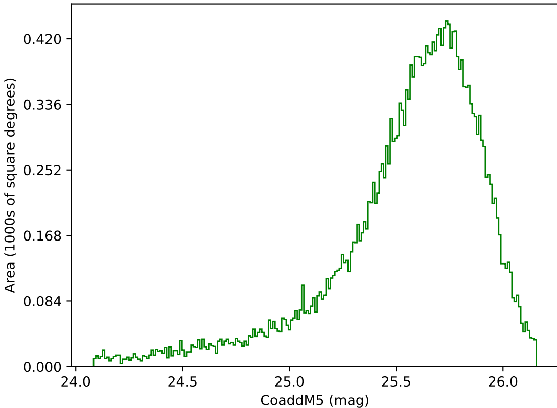
too_elab_r16_d3_griz_v3.4_10yrs Yr 1 g band: CoaddM5
