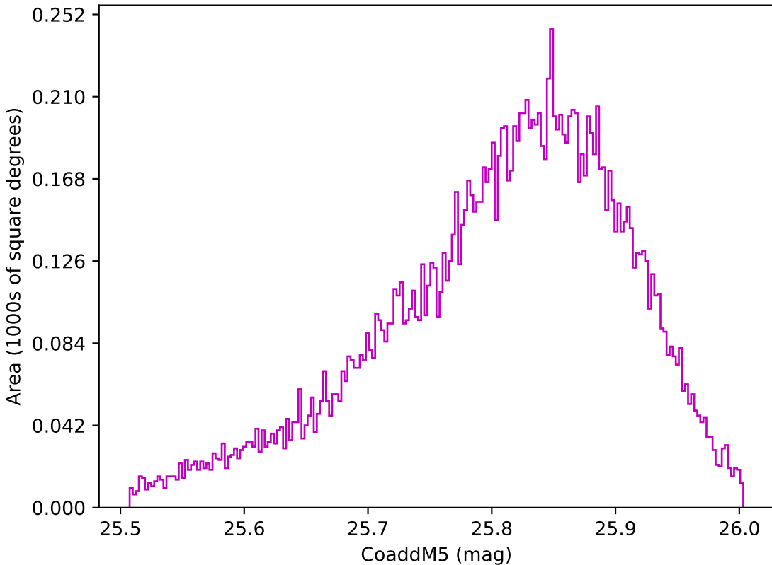
too_elab_r16_d3_griz_v3.4_10yrs WFD z band: CoaddM5
