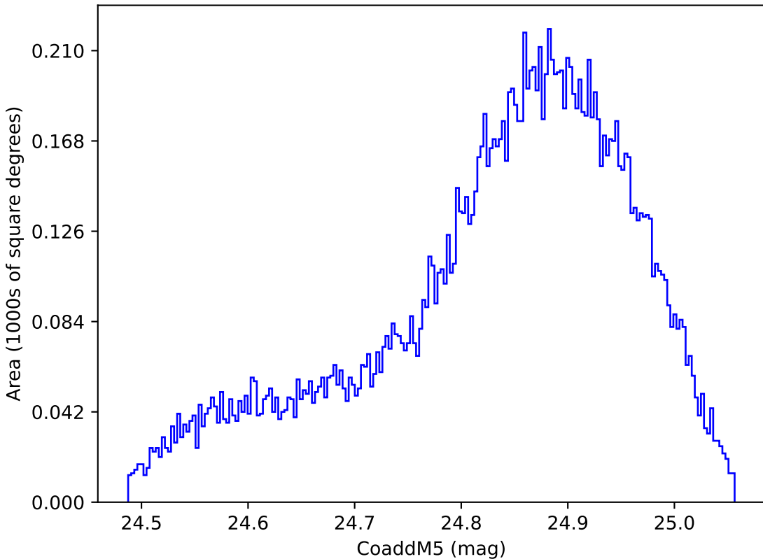
too_elab_r16_d3_griz_v3.4_10yrs WFD y band: CoaddM5
