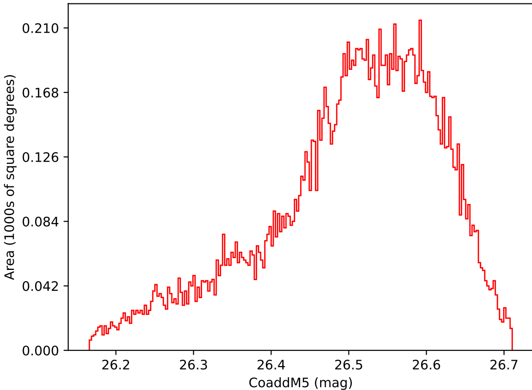
too_elab_r16_d3_griz_v3.4_10yrs WFD i band: CoaddM5
