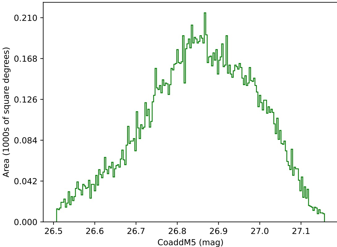
too_elab_r16_d3_griz_v3.4_10yrs WFD g band: CoaddM5
