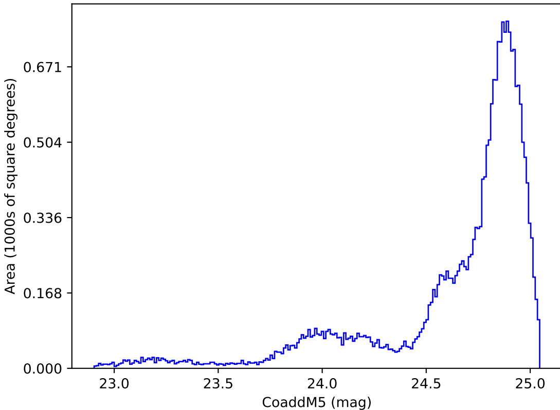
too_elab_r16_d3_griz_v3.4_10yrs All sky y band: CoaddM5
