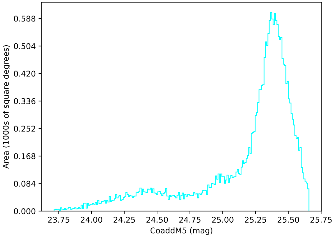
too_elab_r16_d3_griz_v3.4_10yrs All sky u band: CoaddM5
