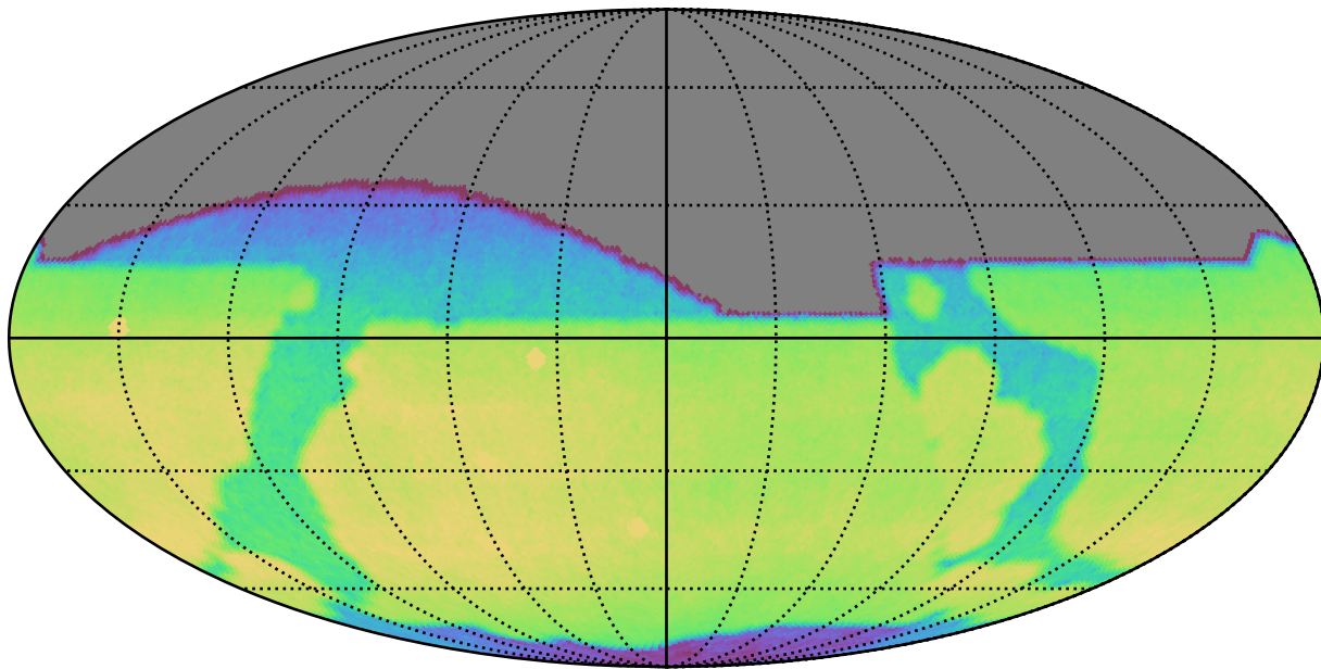
too_elab_r16_d3_griz_v3.4_10yrs All sky r band: CoaddM5
