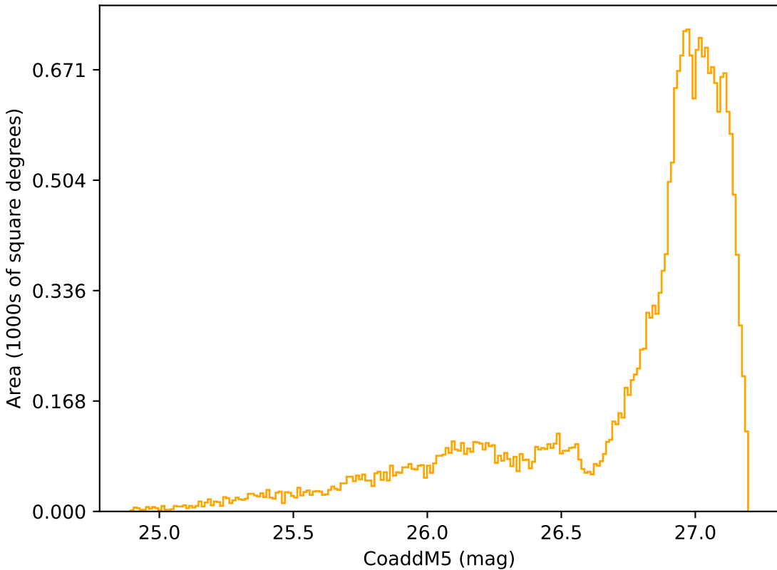
too_elab_r16_d3_griz_v3.4_10yrs All sky r band: CoaddM5
