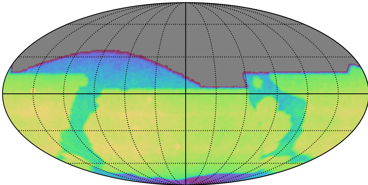
too_elab_r16_d3_griz_v3.4_10yrs All sky i band: CoaddM5
