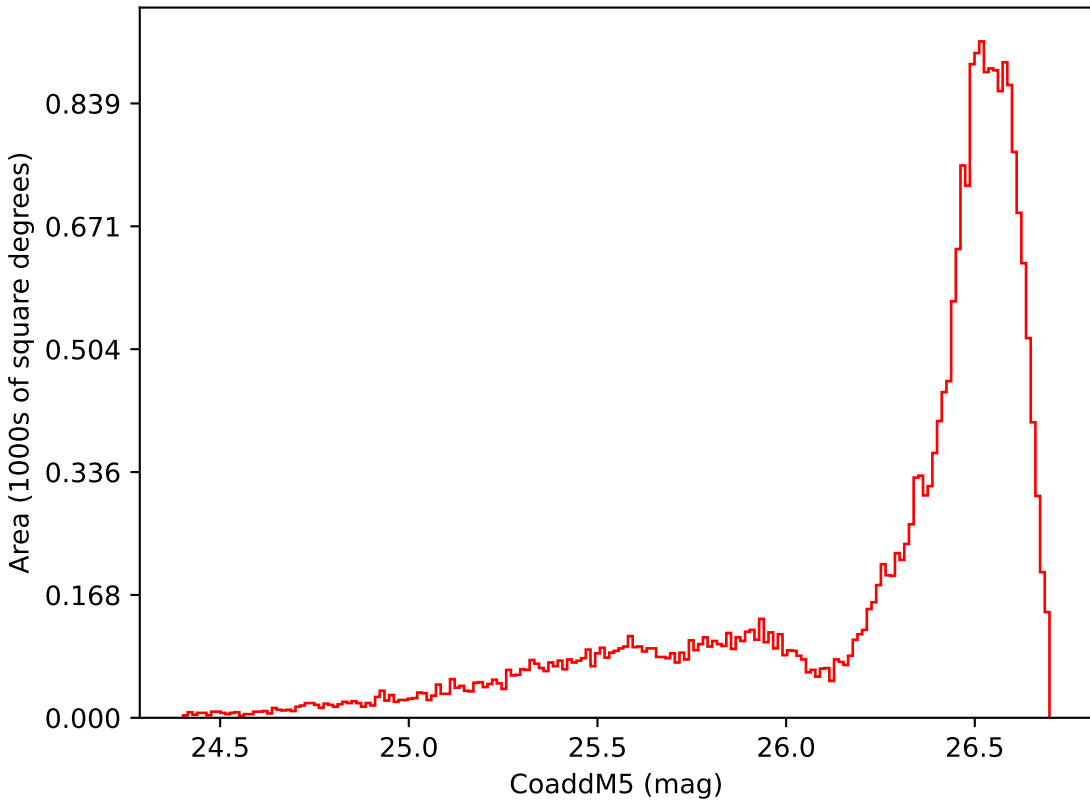
too_elab_r16_d3_griz_v3.4_10yrs All sky i band: CoaddM5
