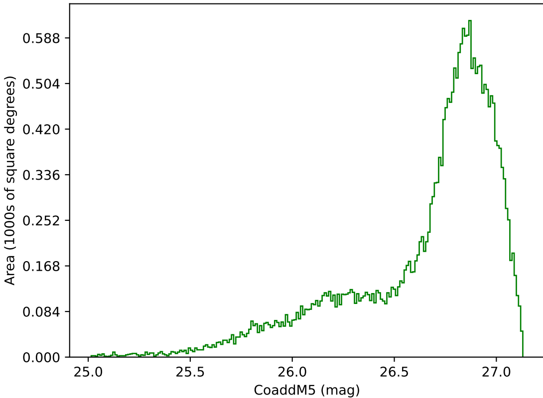
too_elab_r16_d3_griz_v3.4_10yrs All sky g band: CoaddM5
