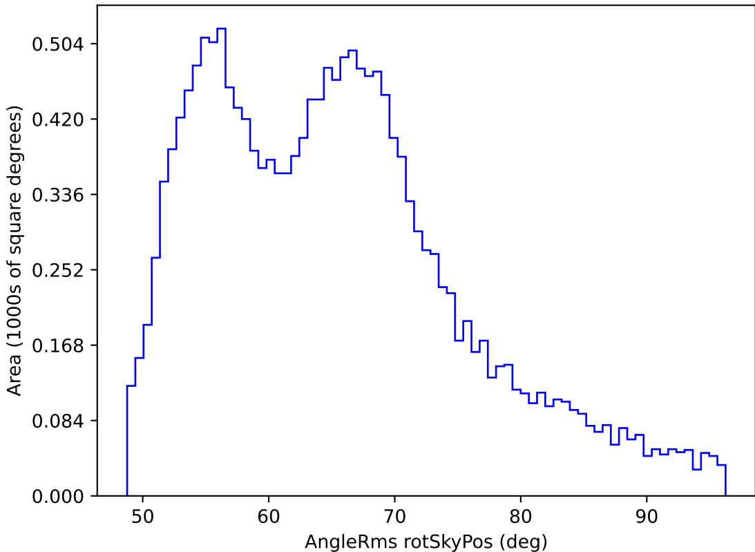
too_elab_r16_d3_griz_v3.4_10yrs WFD z band: AngleRms rotSkyPos
