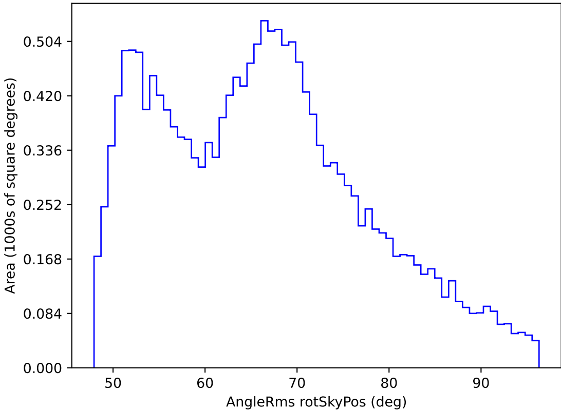
too_elab_r16_d3_griz_v3.4_10yrs WFD r band: AngleRms rotSkyPos
