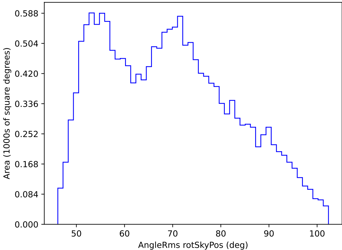
too_elab_r16_d3_griz_v3.4_10yrs WFD g band: AngleRms rotSkyPos
