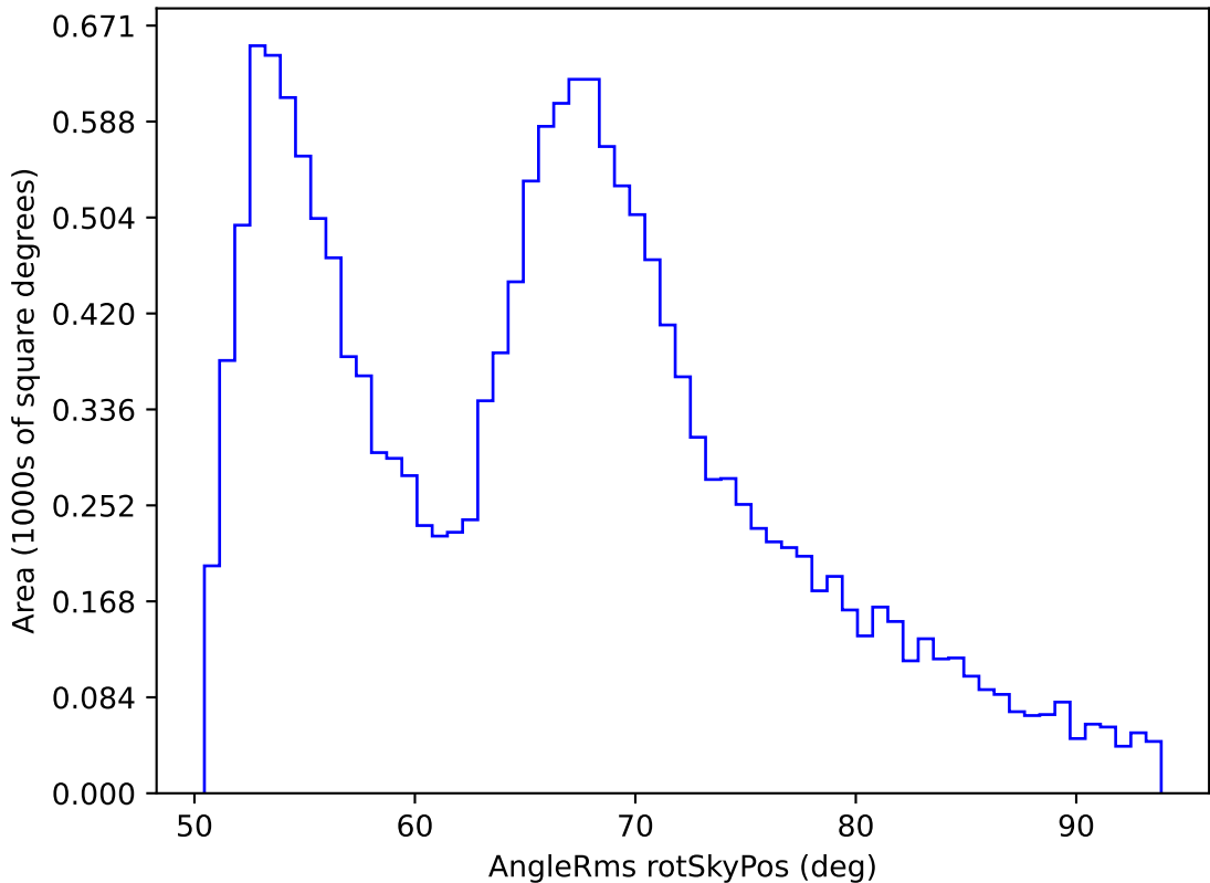
too_elab_r16_d3_griz_v3.4_10yrs WFD all bands: AngleRms rotSkyPos
