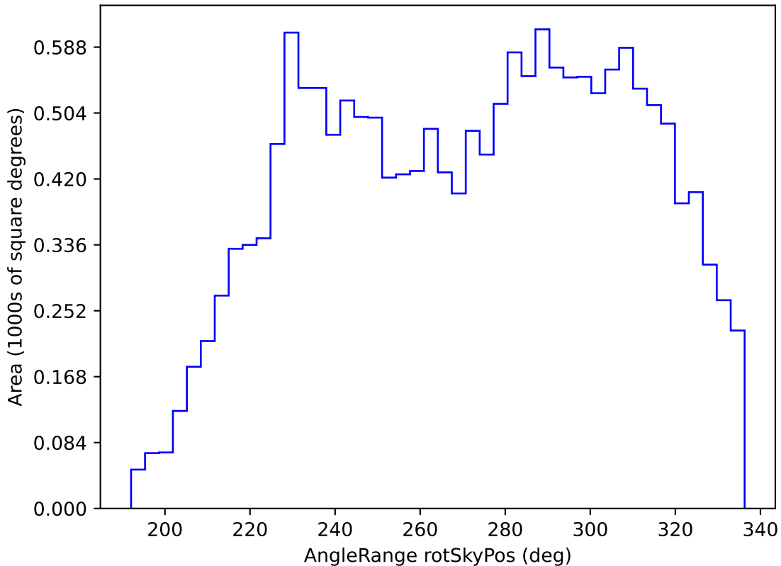
too_elab_r16_d3_griz_v3.4_10yrs WFD y band: AngleRange rotSkyPos
