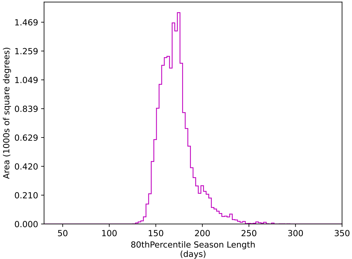
too_elab_r16_d3_griz_v3.4_10yrs WFD z band: 80thPercentile Season Length
