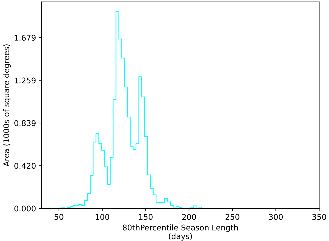
too_elab_r16_d3_griz_v3.4_10yrs WFD u band: 80thPercentile Season Length
