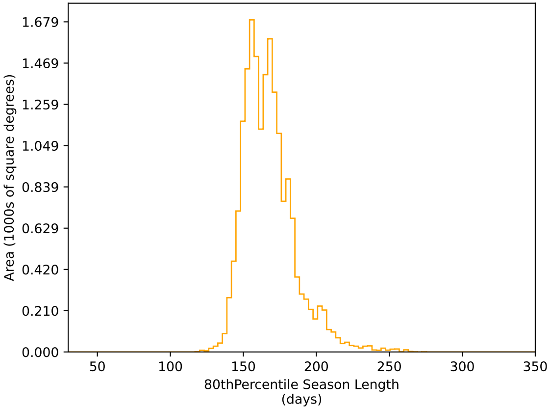
too_elab_r16_d3_griz_v3.4_10yrs WFD r band: 80thPercentile Season Length
