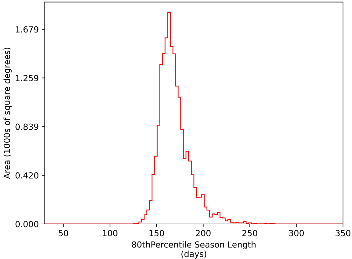
too_elab_r16_d3_griz_v3.4_10yrs WFD i band: 80thPercentile Season Length
