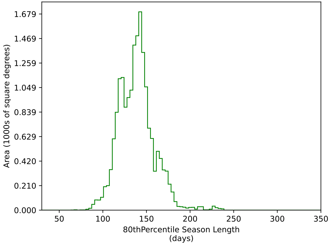
too_elab_r16_d3_griz_v3.4_10yrs WFD g band: 80thPercentile Season Length
