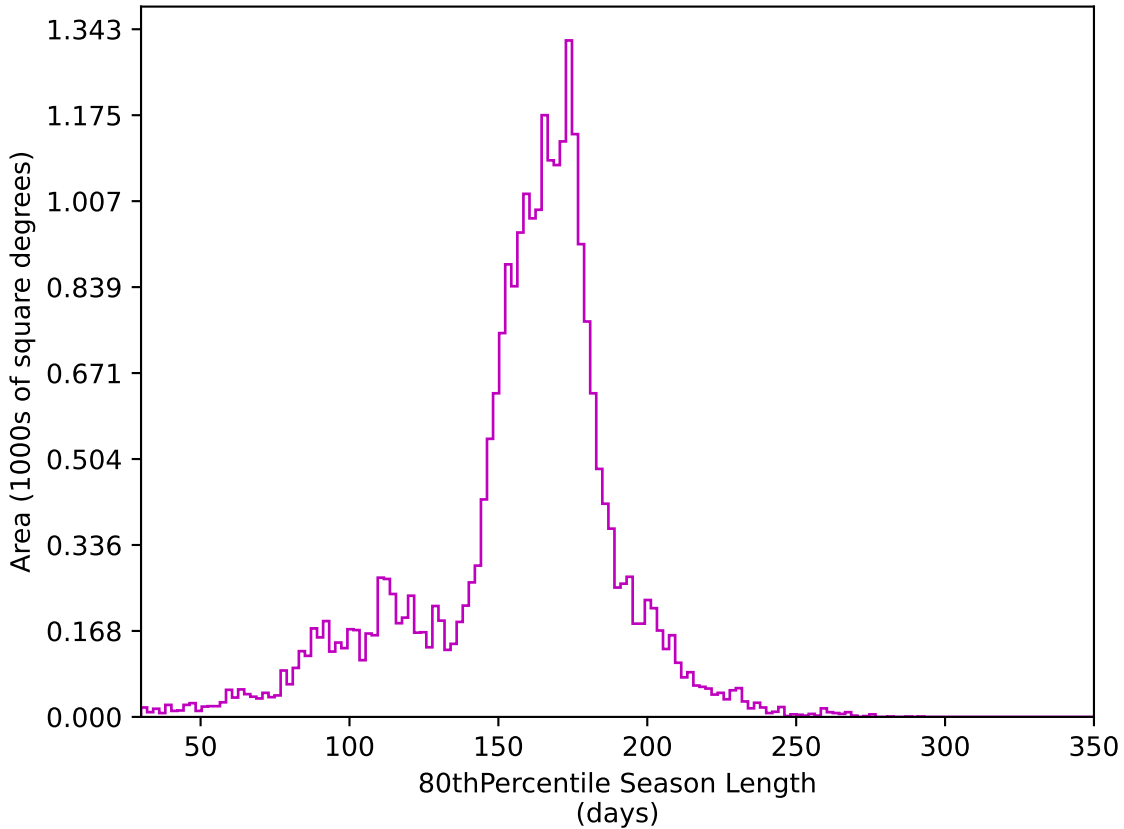
too_elab_r16_d3_griz_v3.4_10yrs All sky z band: 80thPercentile Season Length
