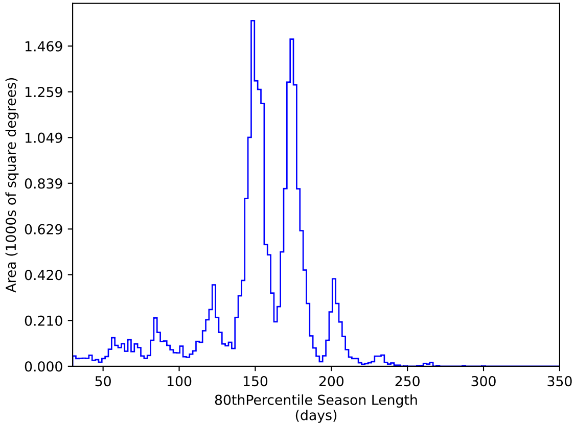
too_elab_r16_d3_griz_v3.4_10yrs All sky y band: 80thPercentile Season Length
