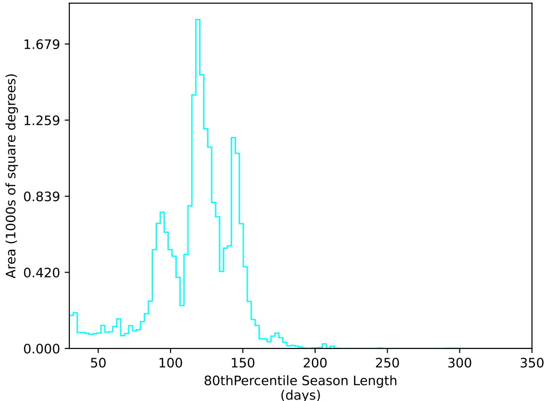
too_elab_r16_d3_griz_v3.4_10yrs All sky u band: 80thPercentile Season Length
