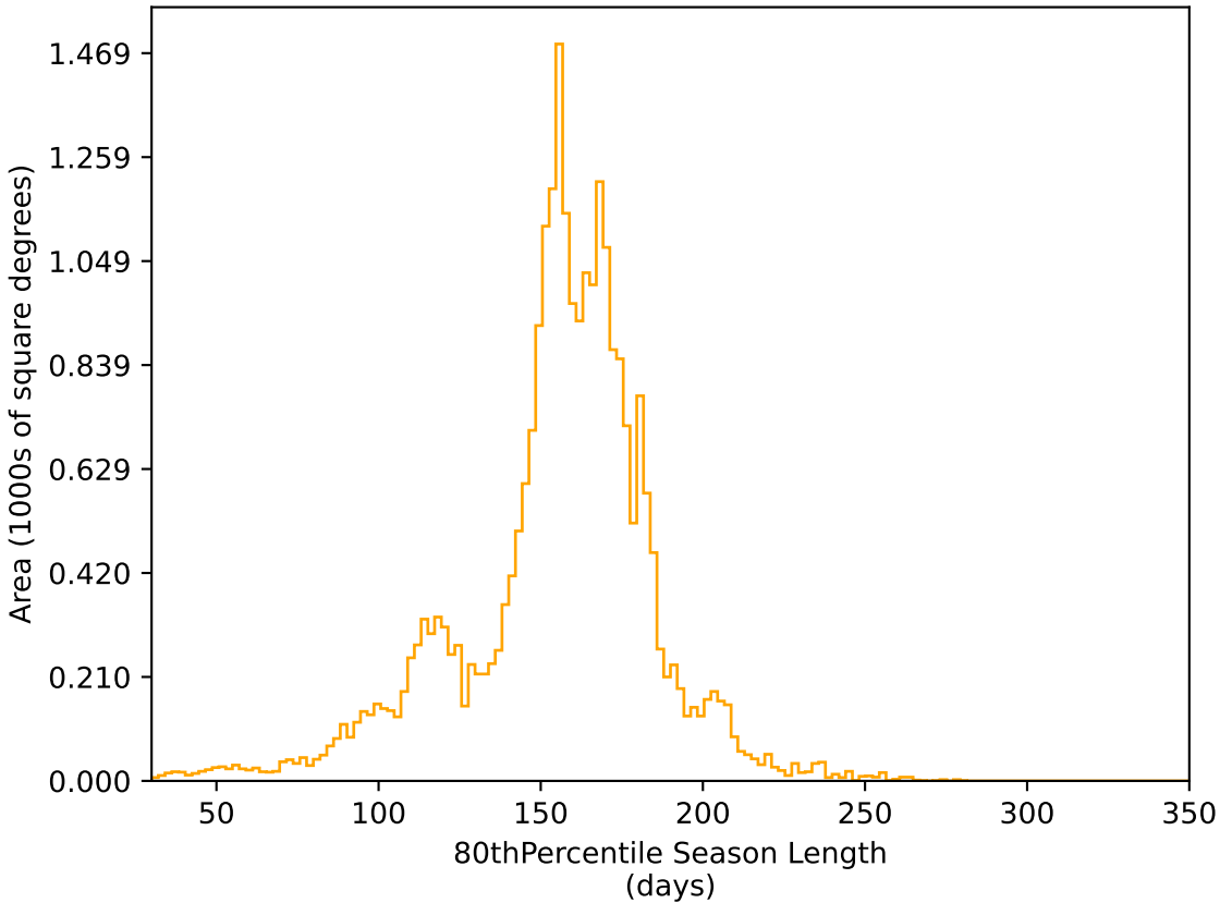
too_elab_r16_d3_griz_v3.4_10yrs All sky r band: 80thPercentile Season Length
