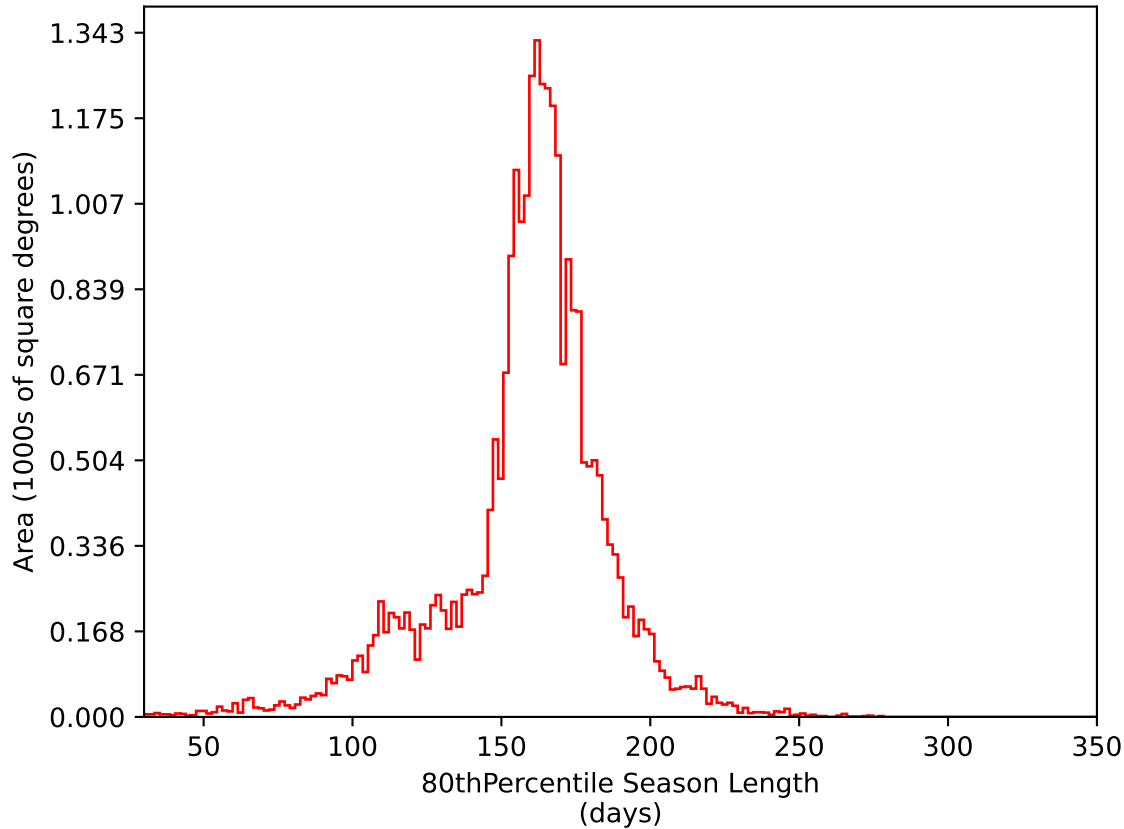
too_elab_r16_d3_griz_v3.4_10yrs All sky i band: 80thPercentile Season Length
