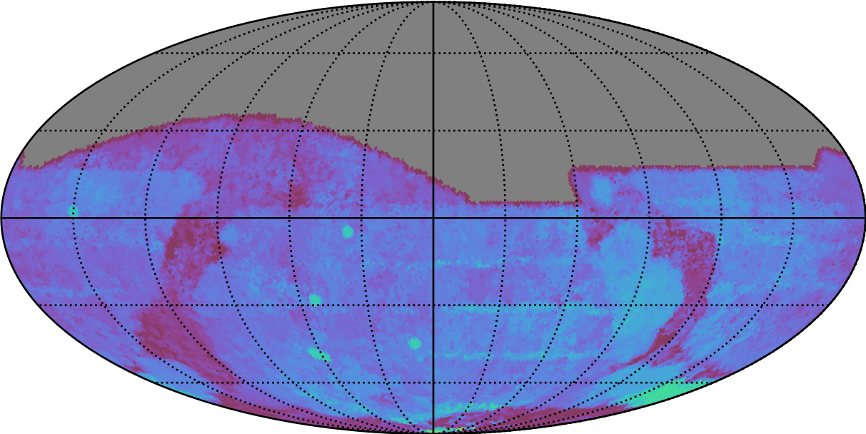
too_elab_r16_d3_griz_v3.4_10yrs All sky g band: 80thPercentile Season Length
