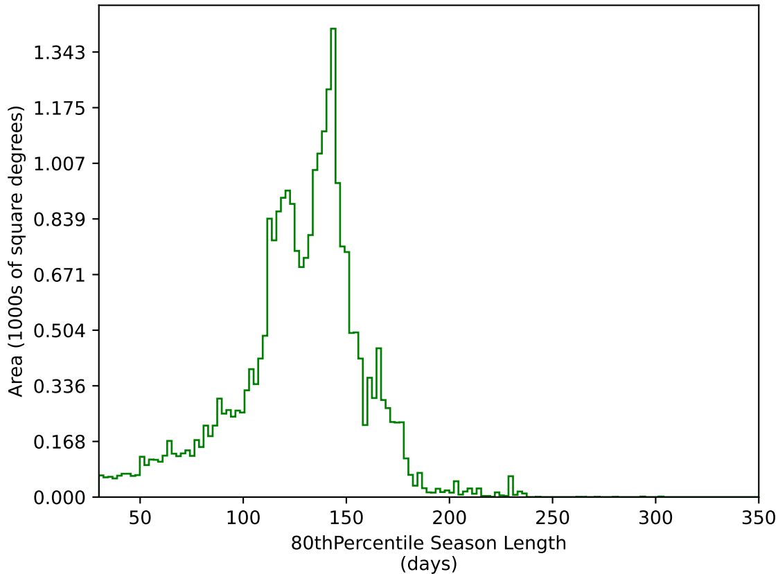
too_elab_r16_d3_griz_v3.4_10yrs All sky g band: 80thPercentile Season Length
