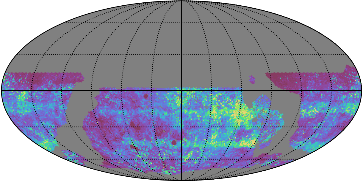
too_elab_r16_d3_griz_v3.4_10yrs WFD zy bands: 75th Percentile Intranight Timespan
