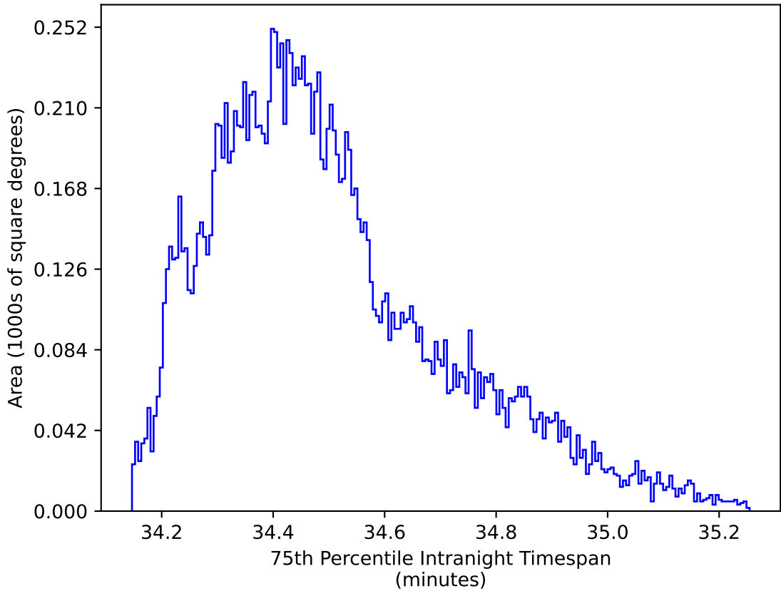
too_elab_r16_d3_griz_v3.4_10yrs WFD zy bands: 75th Percentile Intranight Timespan
