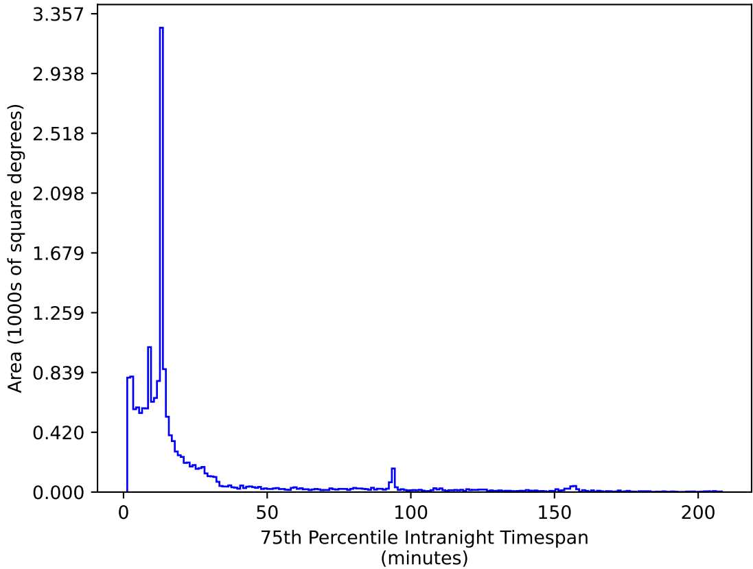
too_elab_r16_d3_griz_v3.4_10yrs WFD z band: 75th Percentile Intranight Timespan
