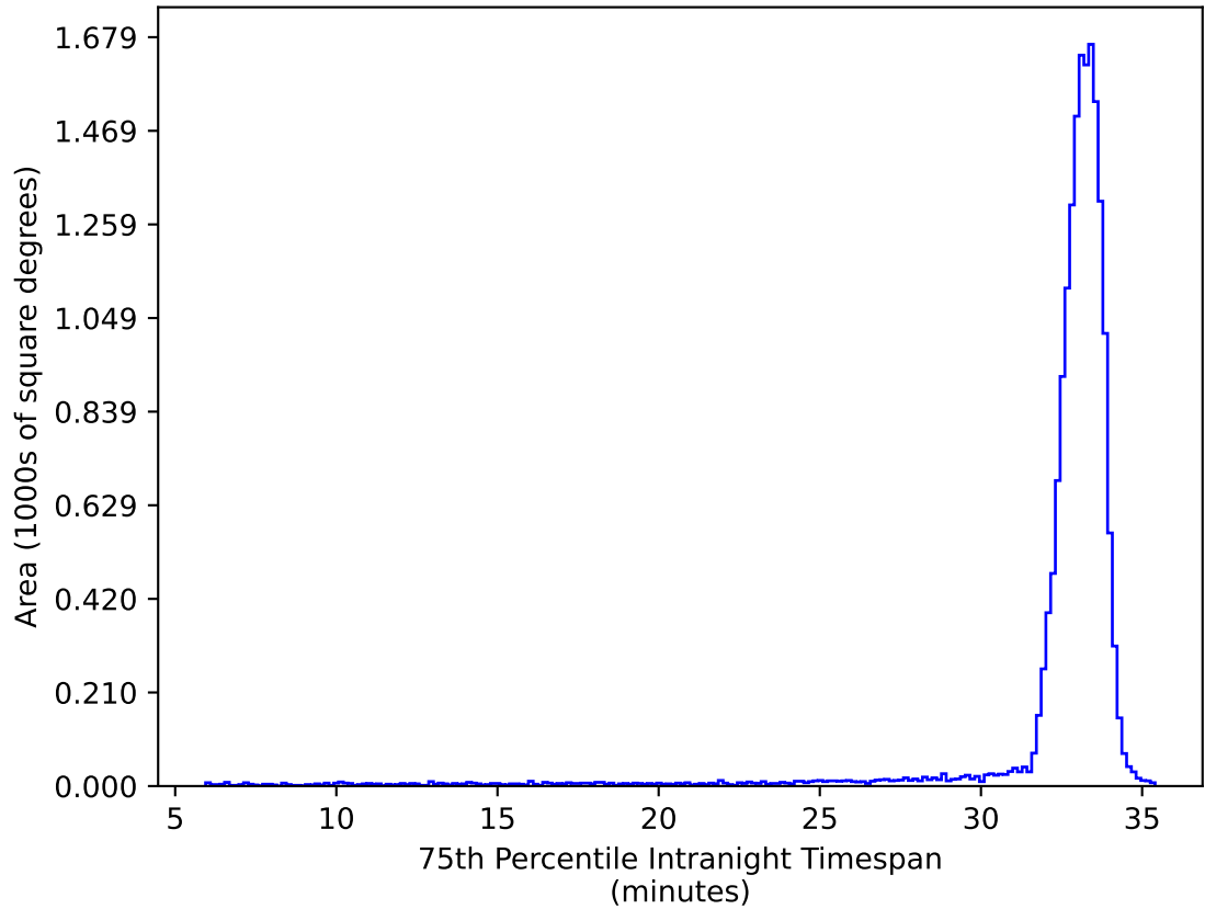
too_elab_r16_d3_griz_v3.4_10yrs WFD ug bands: 75th Percentile Intranight Timespan
