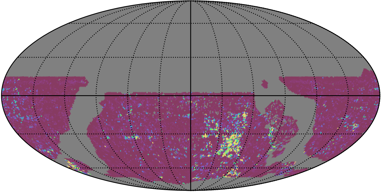
too_elab_r16_d3_griz_v3.4_10yrs WFD u band: 75th Percentile Intranight Timespan
