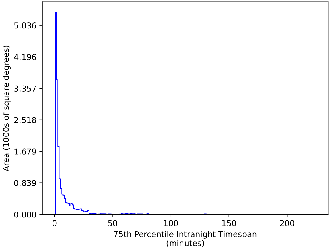
too_elab_r16_d3_griz_v3.4_10yrs WFD u band: 75th Percentile Intranight Timespan
