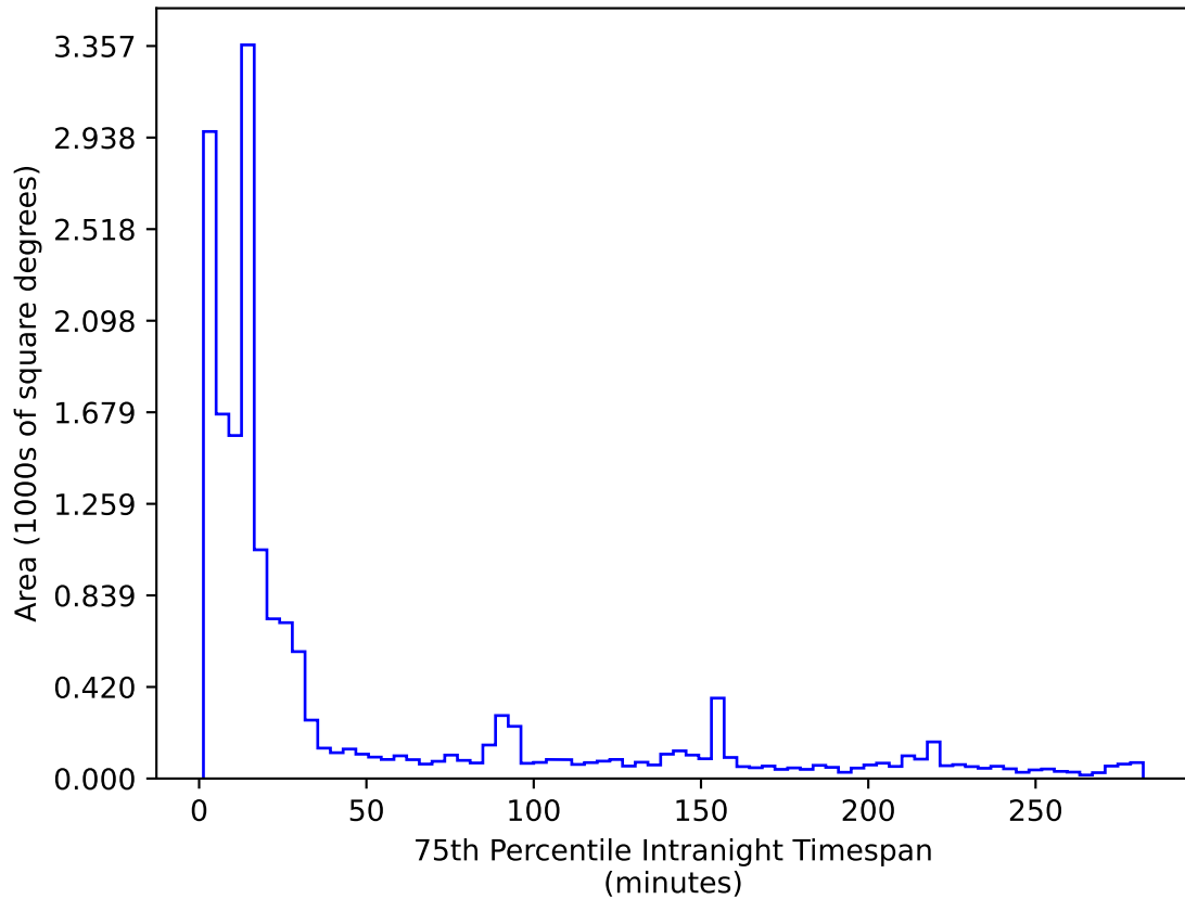
too_elab_r16_d3_griz_v3.4_10yrs WFD r band: 75th Percentile Intranight Timespan
