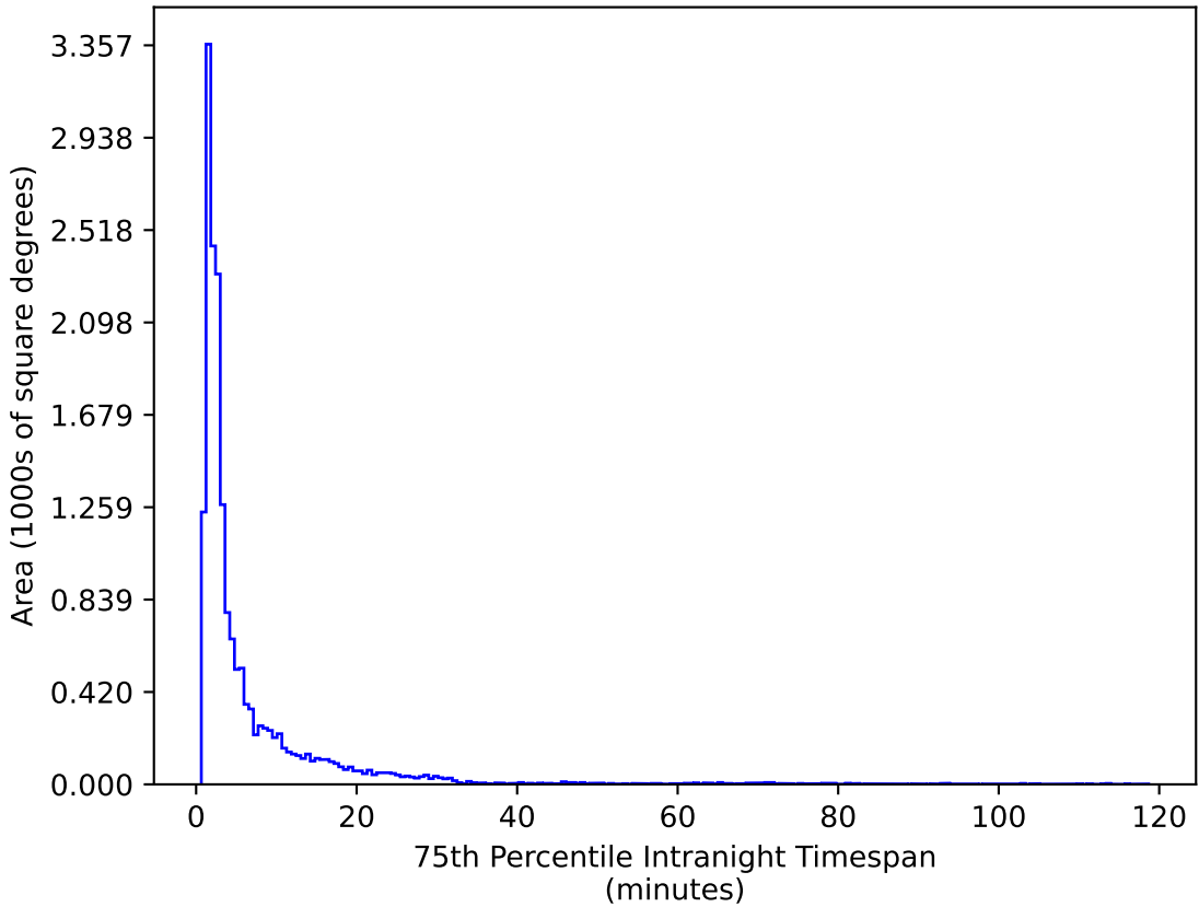
too_elab_r16_d3_griz_v3.4_10yrs WFD g band: 75th Percentile Intranight Timespan
