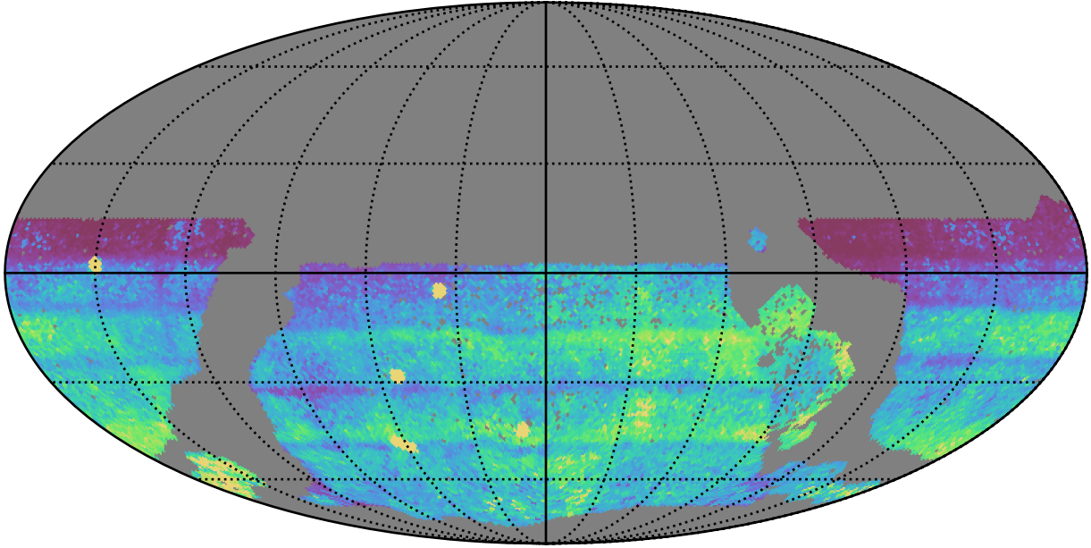
too_elab_r16_d3_griz_v3.4_10yrs WFD all bands: 75th Percentile Intranight Timespan
