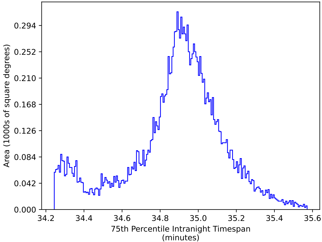
too_elab_r16_d3_griz_v3.4_10yrs WFD all bands: 75th Percentile Intranight Timespan
