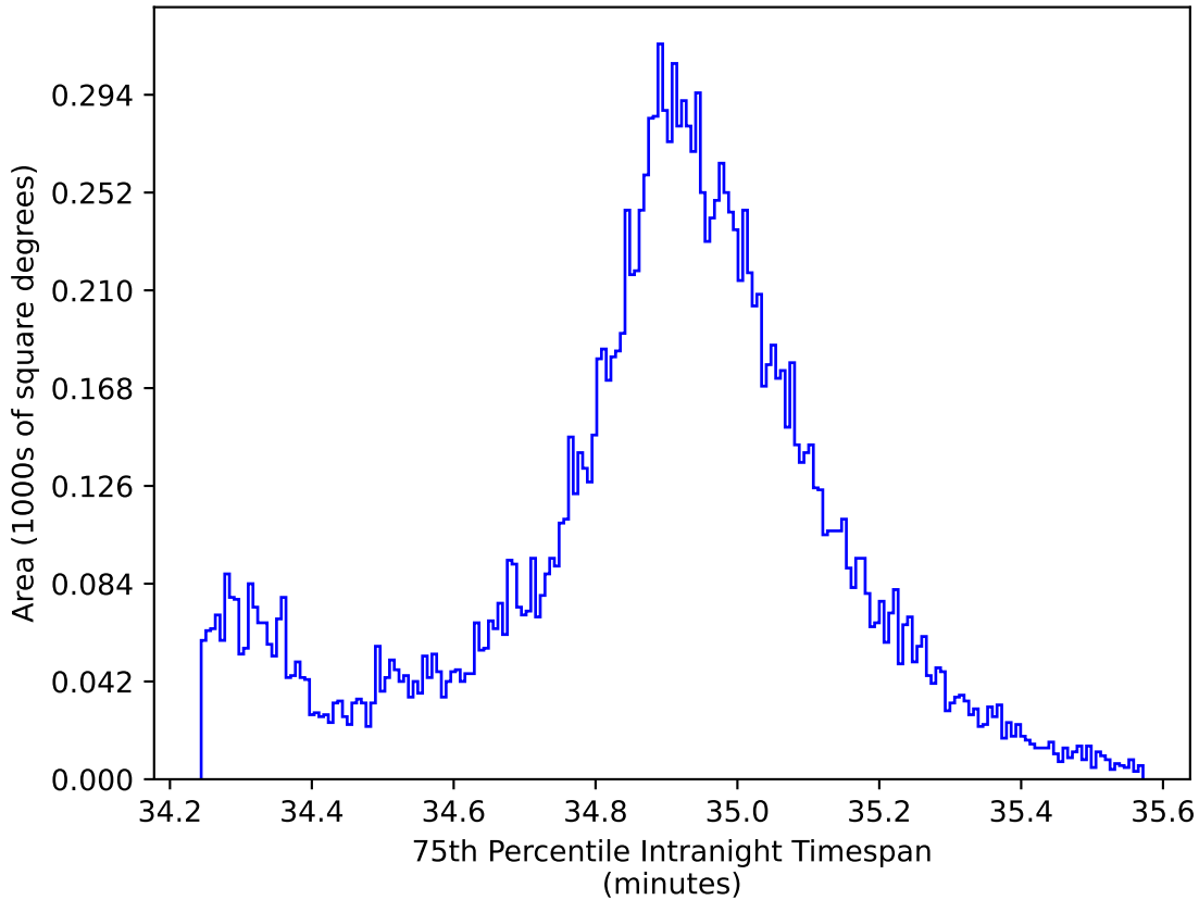
too_elab_r16_d3_griz_v3.4_10yrs WFD: 75th Percentile Intranight Timespan
