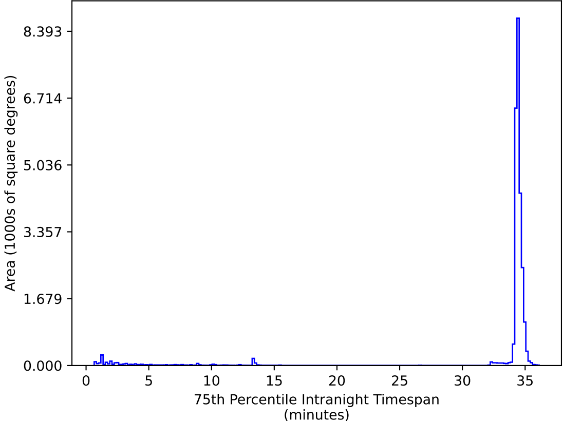
too_elab_r16_d3_griz_v3.4_10yrs All sky zy bands: 75th Percentile Intranight Timespan
