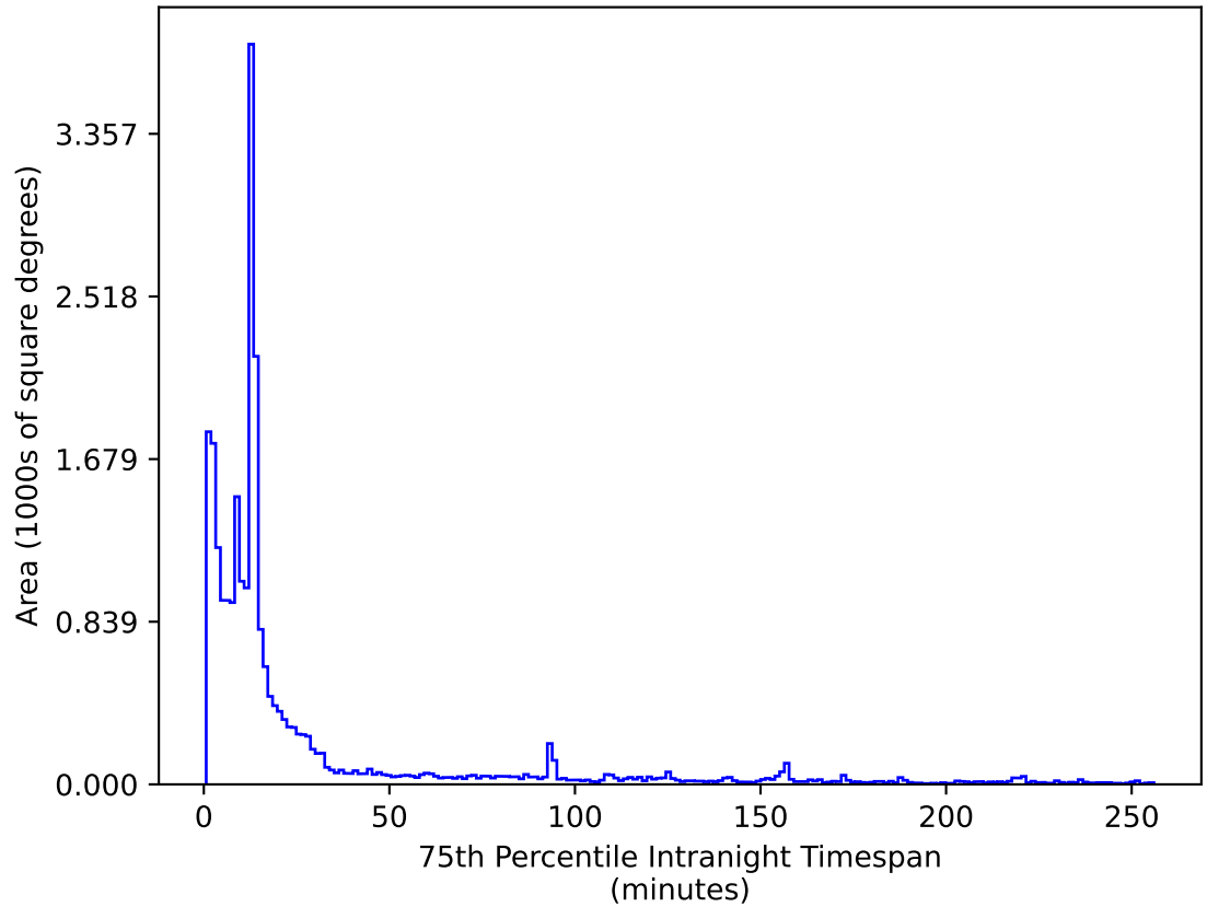
too_elab_r16_d3_griz_v3.4_10yrs All sky z band: 75th Percentile Intranight Timespan
