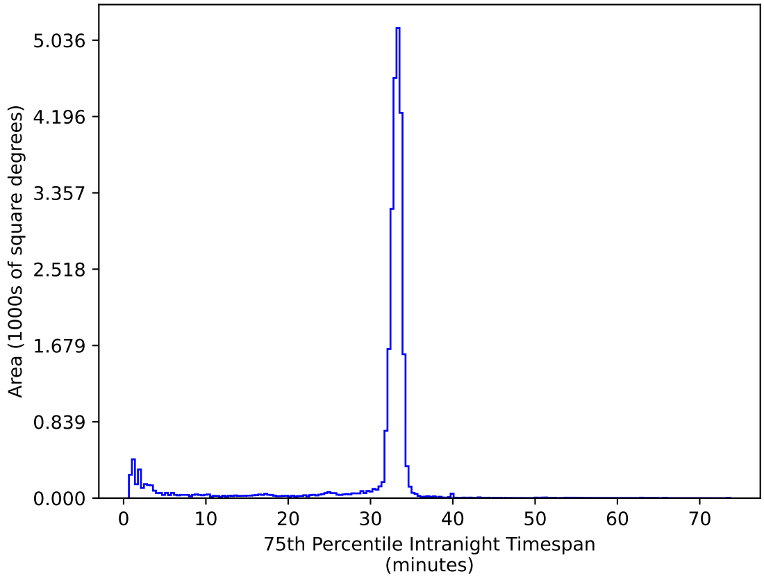
too_elab_r16_d3_griz_v3.4_10yrs All sky ug bands: 75th Percentile Intranight Timespan
