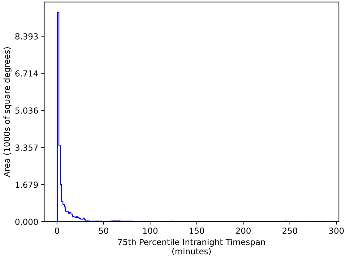
too_elab_r16_d3_griz_v3.4_10yrs All sky u band: 75th Percentile Intranight Timespan
