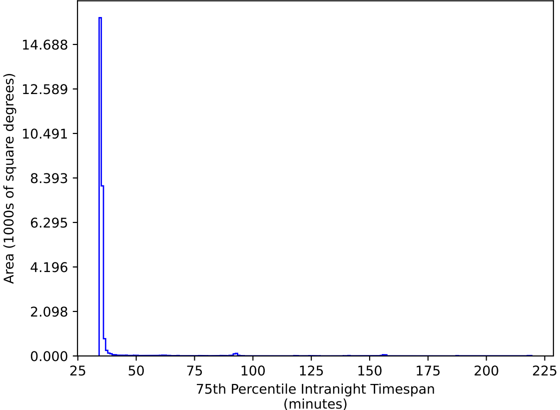
too_elab_r16_d3_griz_v3.4_10yrs All sky ri bands: 75th Percentile Intranight Timespan
