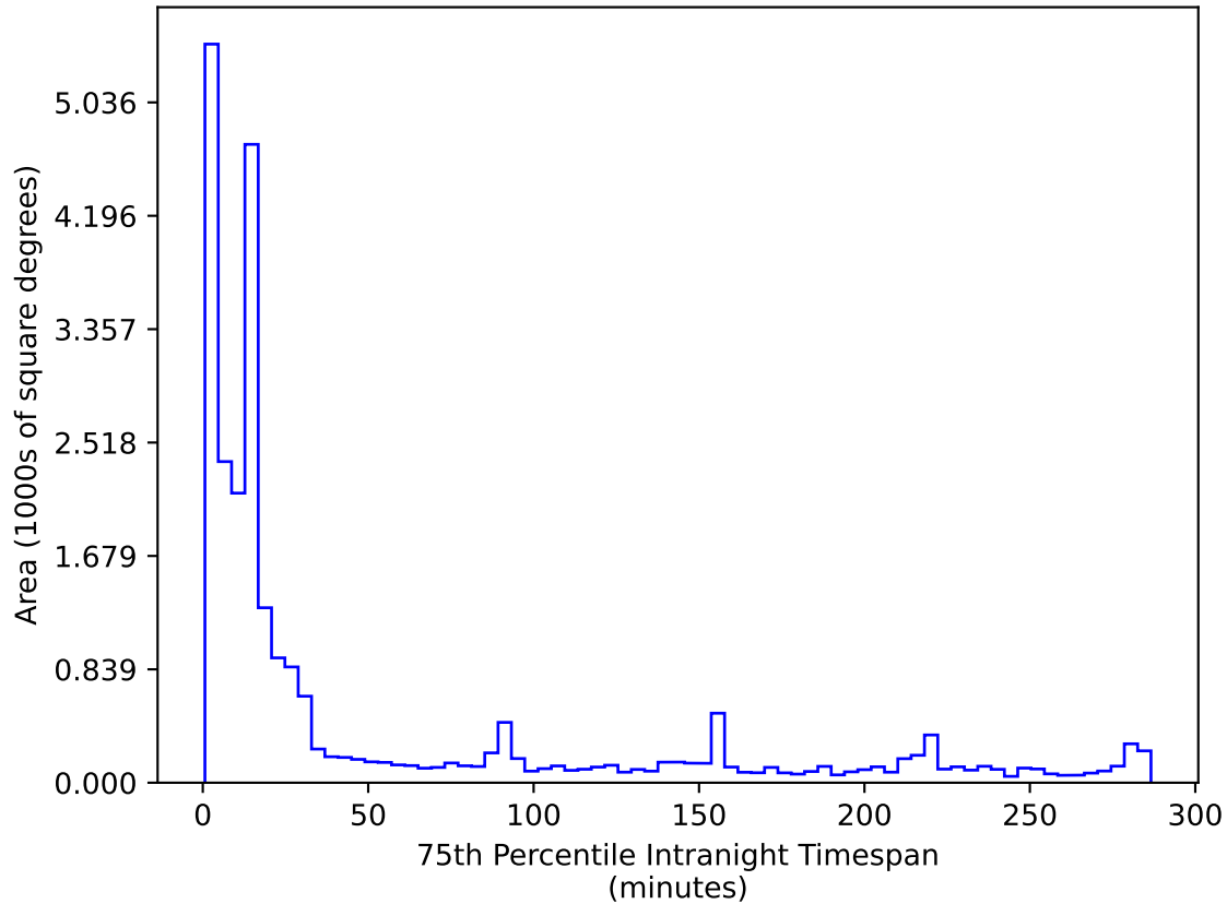
too_elab_r16_d3_griz_v3.4_10yrs All sky r band: 75th Percentile Intranight Timespan
