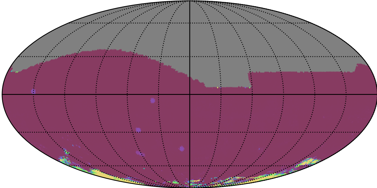
too_elab_r16_d3_griz_v3.4_10yrs All sky iz bands: 75th Percentile Intranight Timespan
